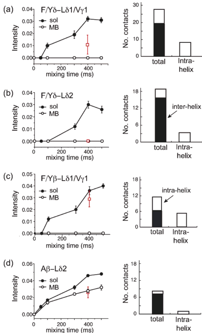
Figure 4. 13 C spin diffusion buildup curves for inter-residue cross-peaks (left column) and the corresponding numbers of intrahelical (open) and interhelical (filled) contacts within 5.5 Å in the soluble colicin structure (right column). The cross-peaks are (a) F/Yδ-Lδ1/Vγ1, (b) F/Yδ-Lδ2, (c) F/Yβ-Lδ1/Vγ1, and (d) Aβ-Lδ2. Filled circles represent the soluble colicin data at 292 K. Open circles and red open squares represent the MB colicin data at 292 and 243 K, respectively.
