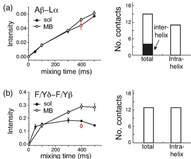
Figure 5. 13 C spin diffusion buildup curves (left column) and the numbers of interhelical and intrahelical contacts within 5.5 Å in the soluble colicin structure. (a) Aβ-Lα. (b) F/Yδ-F/Yβ. Symbols are the same as those in Figure 4. At room temperature, the MB protein exhibits similar or faster spin diffusion than the soluble protein due to the predominance of intrahelical contacts and the large diffusion coefficient.
